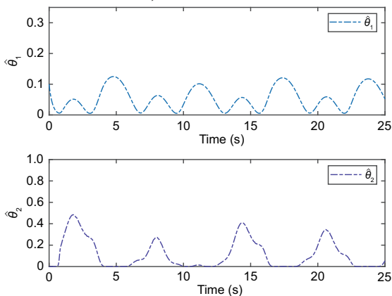
Fig. 6 Curves of \hat{\theta}_i ( i = 1, 2 )
