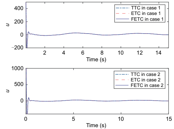
Fig. 3 Curves of the control input under cases 1 and 2 (ETC: event-triggered control; FETC: fixed-threshold ETC; TTC: time-triggered control)
