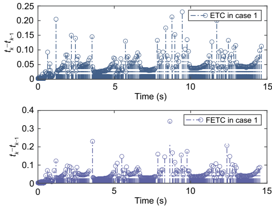
Fig. 4 Triggering instants and inter-event intervals under case 1 (ETC: event-triggered control; FETC: fixed-threshold ETC)
