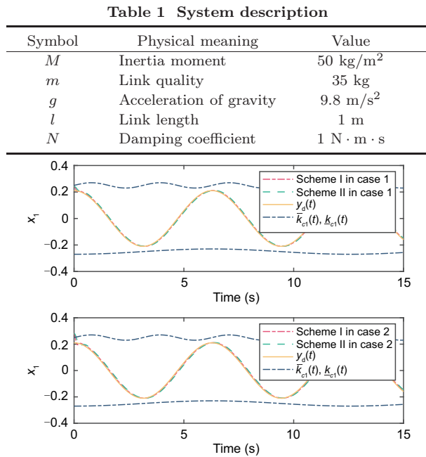
Fig. 1 Curves of x_1 and y_d(t) with Schemes I and II under cases 1 and 2 (Scheme I: the designed method; Scheme II: Zhao et al. (2022)'s method)
