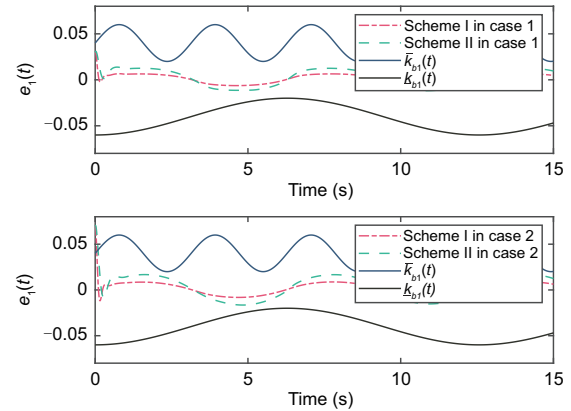
Fig. 2 Curves of the tracking error e_1(t) with Schemes I and II under cases 1 and 2 (Scheme I: the designed method; Scheme II: Zhao et al. (2022)'s method)
